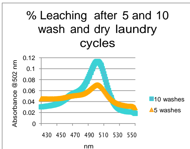
Fig 8. Vex-Protex-All™ showed remarkable binding strength and stability even after repeated wash cycles in an industrial laundry facility. The percentage loss of the molecule was calculated to be on average 0.106% / wash cycle or 0.53% after 10 cycles.
